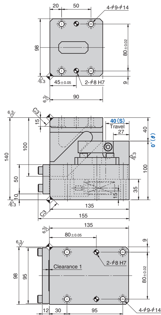
● Cam Diagram
