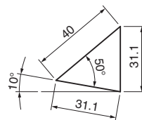
● Cam Diagram
