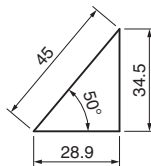
● Cam Diagram
