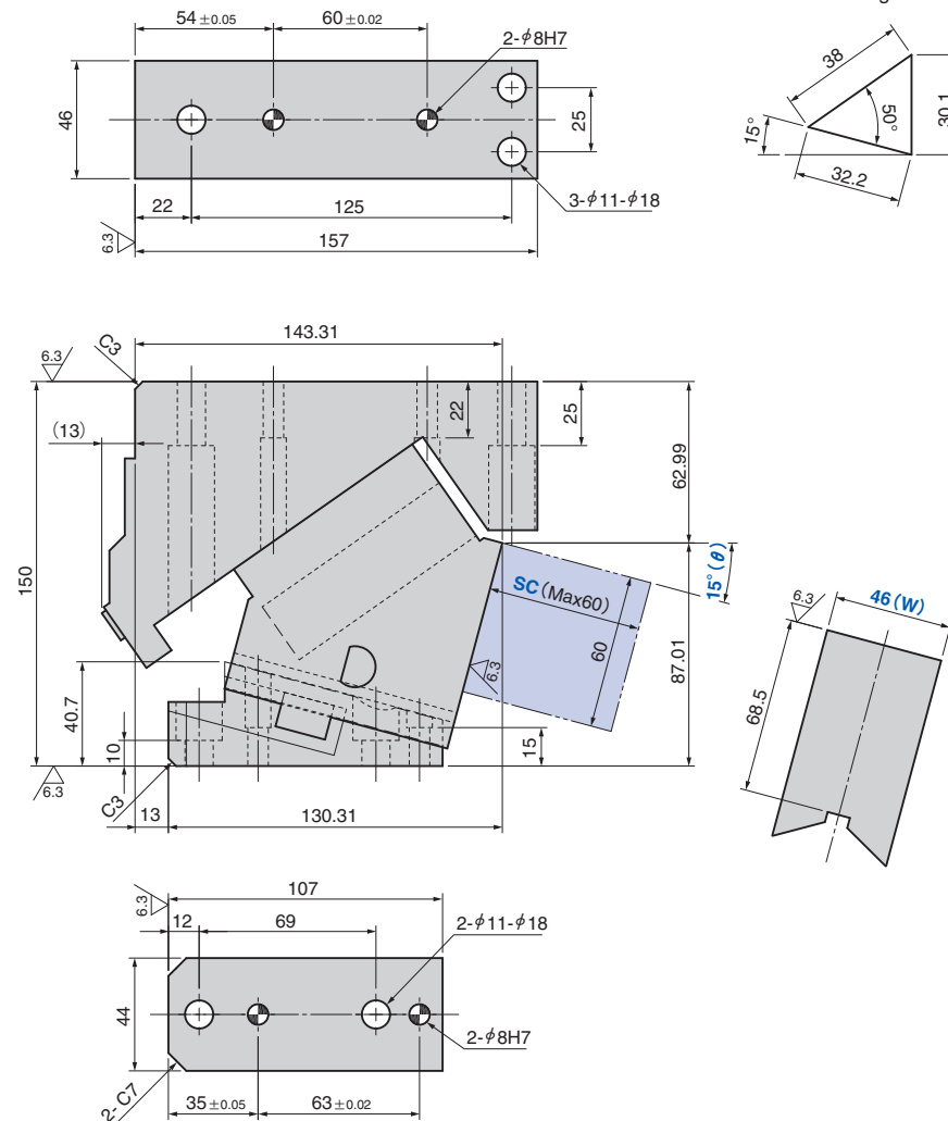
● Cam Diagram
