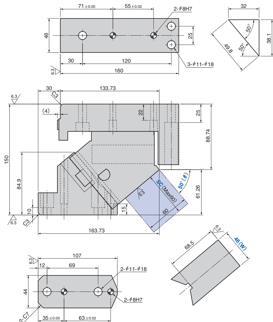
● Cam Diagram
