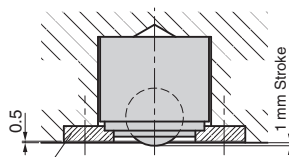
Inverted Mount Specification For set plate
