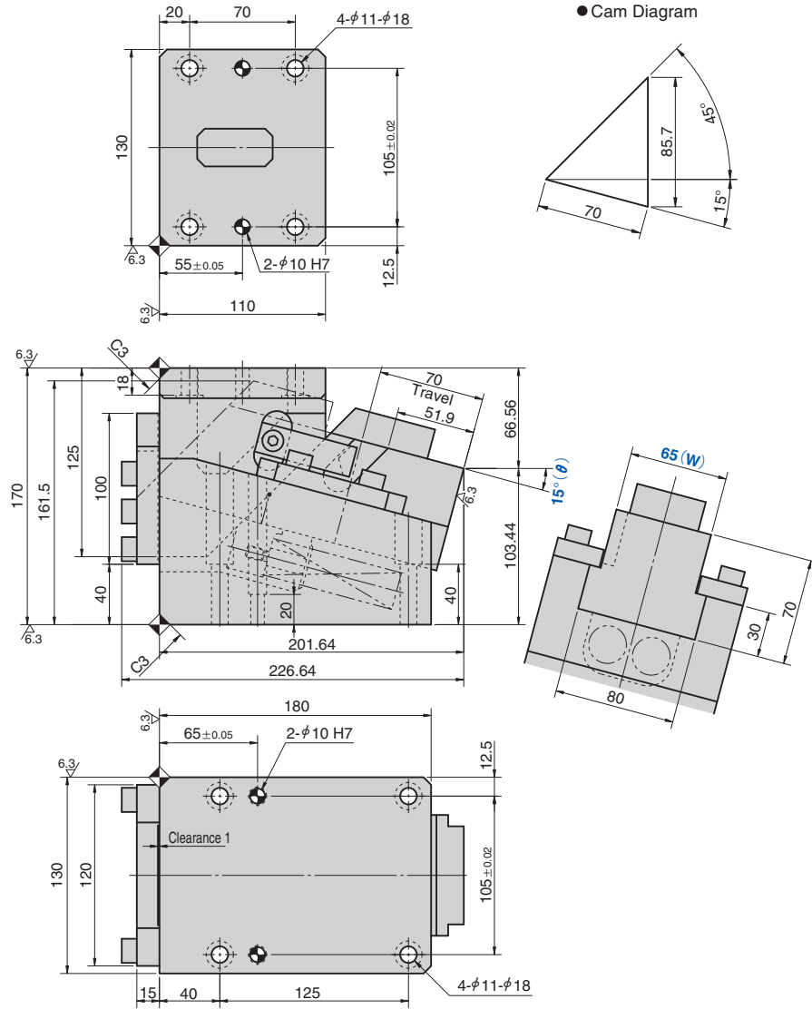
● Cam Diagram
