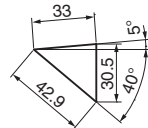
Cam Diagram
