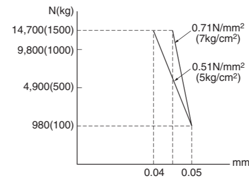
Air lift h (theoretical value)
