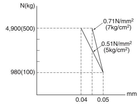
Air lift h (theoretical value)
