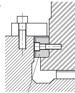
Cam Slide Plate VG2
