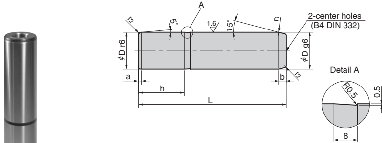
GP DIN9833-D x L (Hanging tap type)
