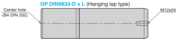
GP DIN9833-D x L (Hanging tap type)
