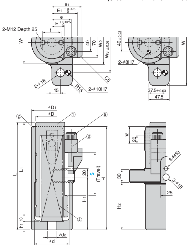
SBLSN (Slide Pin With Dowel Pin Hole)
