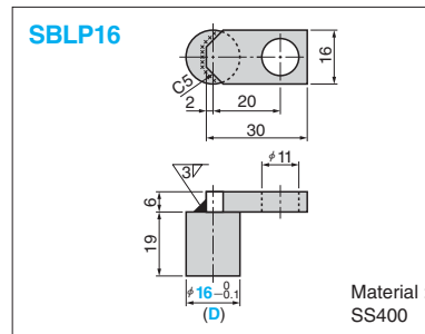
Lock Pin
