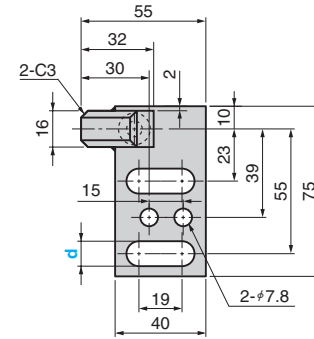
NGLR NGLSR (Gauge Hardening Type)
