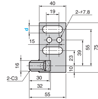
NGLL NGLSL (Gauge Hardening Type)
