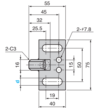
NGLA NGLSA (Gauge Hardening Type)
